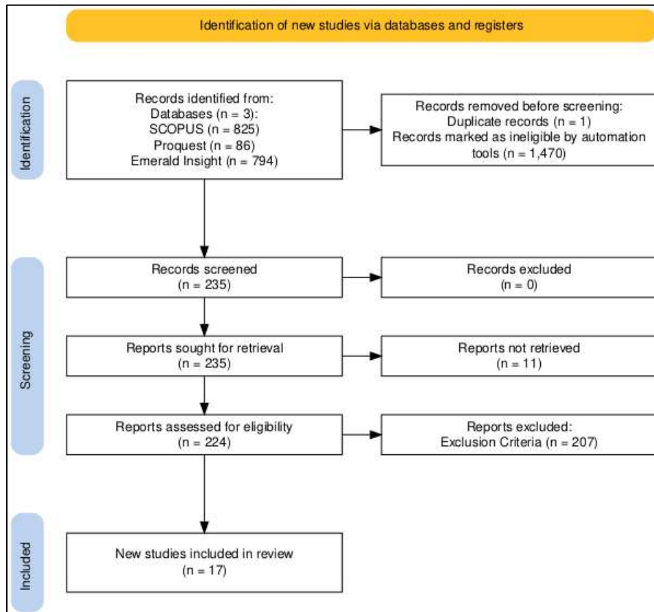
Fig.1. PRISMA Model
